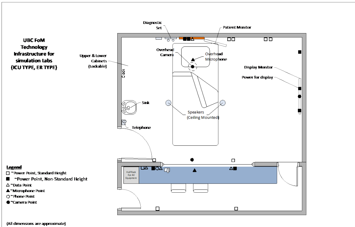
Figure 3: Enhanced Clinical Skills and control-observation room floor plan layout
